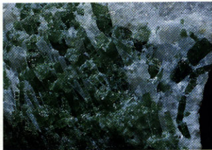
Figure 11. The Panjshir emerald crystals are commonly found in quartz (here, from the Buzmal mine). It is not unusual to find literally hundreds of small crystals in a single block. Photo by Gary Bowersox.
