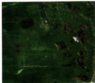
Figure 14. Rhombohedra of what appeared to be a limonite-stained carbonate were found near the surface of one of the Panjshir emeralds examined. Photomicrograph by John I. Koivula, magnified 5 \times .
