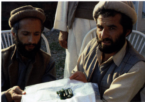
Figure 12. Large emerald crystals are not uncommon in the Panjshir mines. The crystals shown here range up to 132 ct. Photo by Gary Bowersox.
